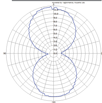
Orientation Read Range (m)
